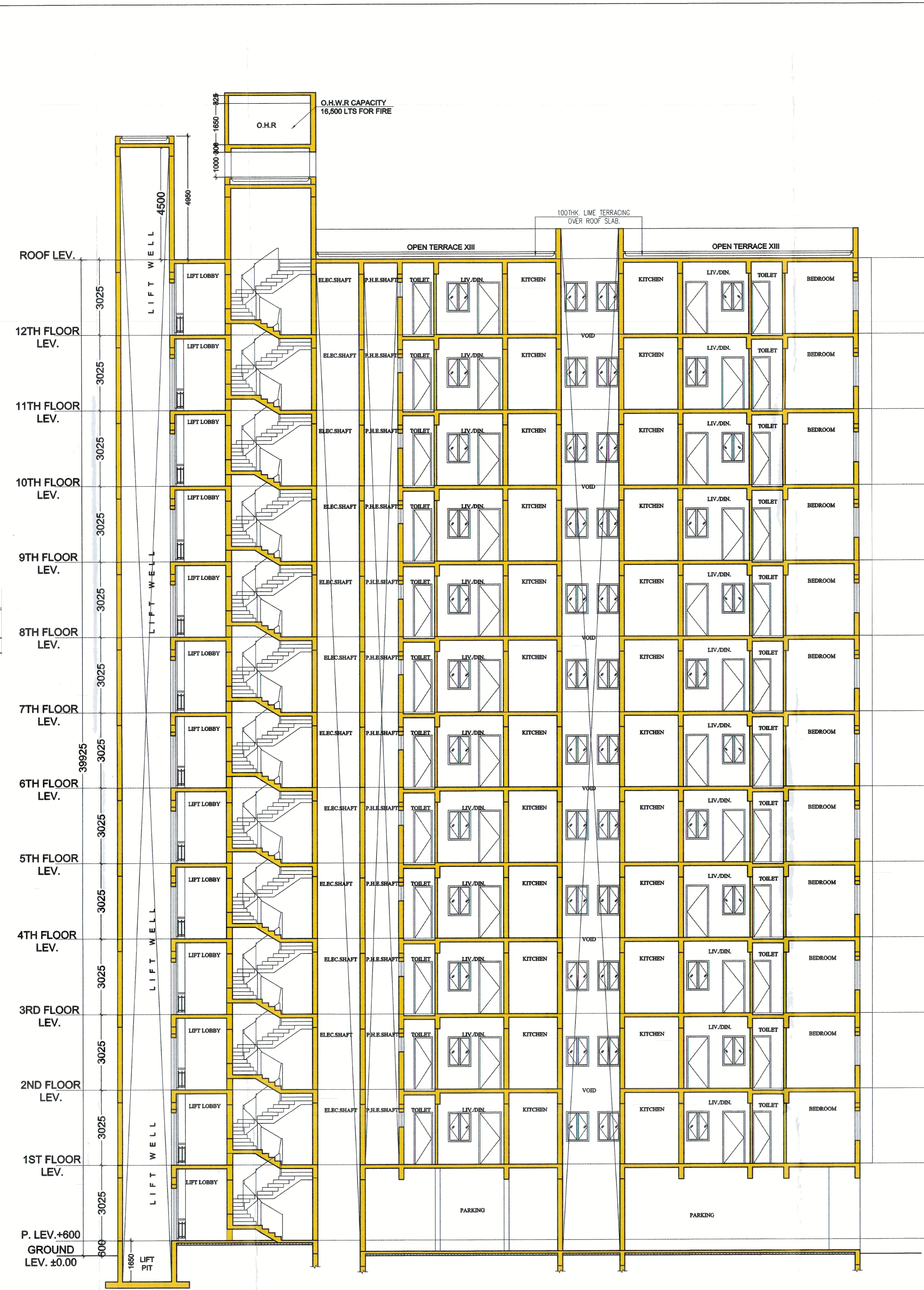
SECTION-BB (BLOCK-C)
